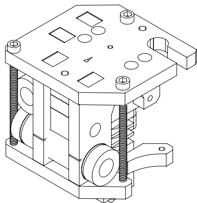
Pre-assembled Carriage with Hotend
